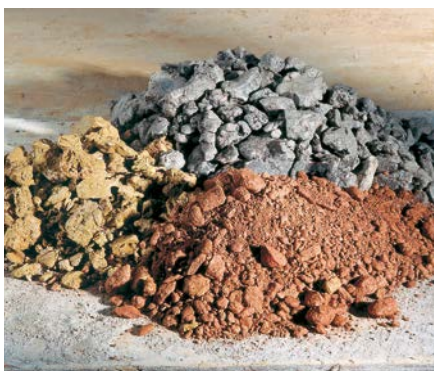
▲ Tonerden
